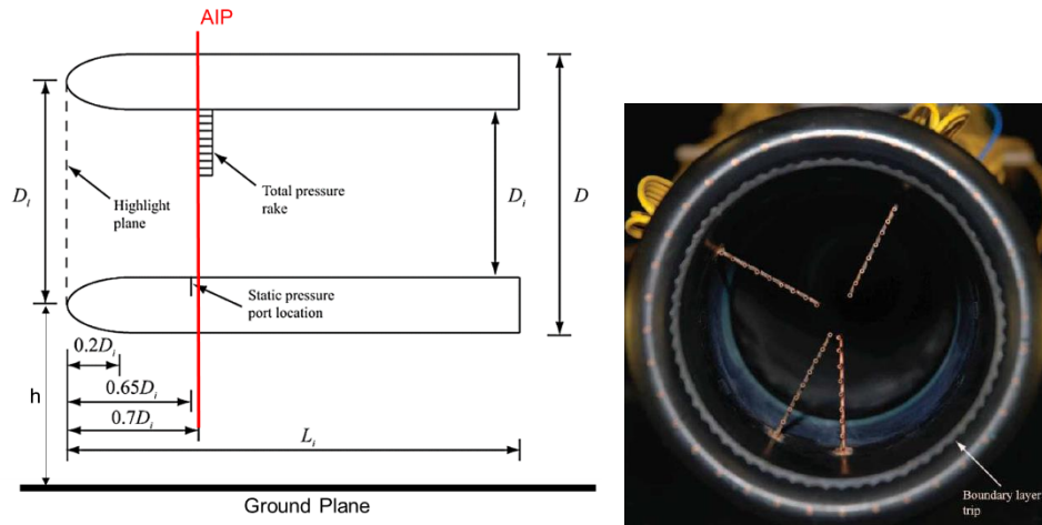
Figure 1.—Experimental configuration for axisymmetric inlet with inner diameter of 100mm and a lip diameter of 120mm. Total pressure is measured with 4 rakes each with 9 probes. The assembly is rotated in order to increase the measurement resolution at the AIP.
